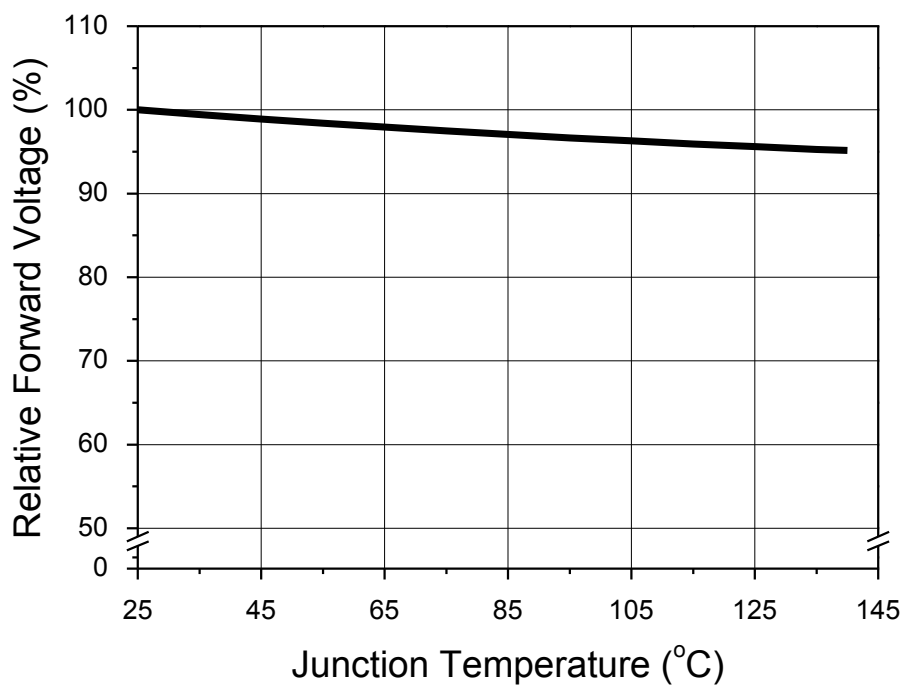
Fig 7. Junction Temperature vs. Forward Voltage, I_F=0.9A
