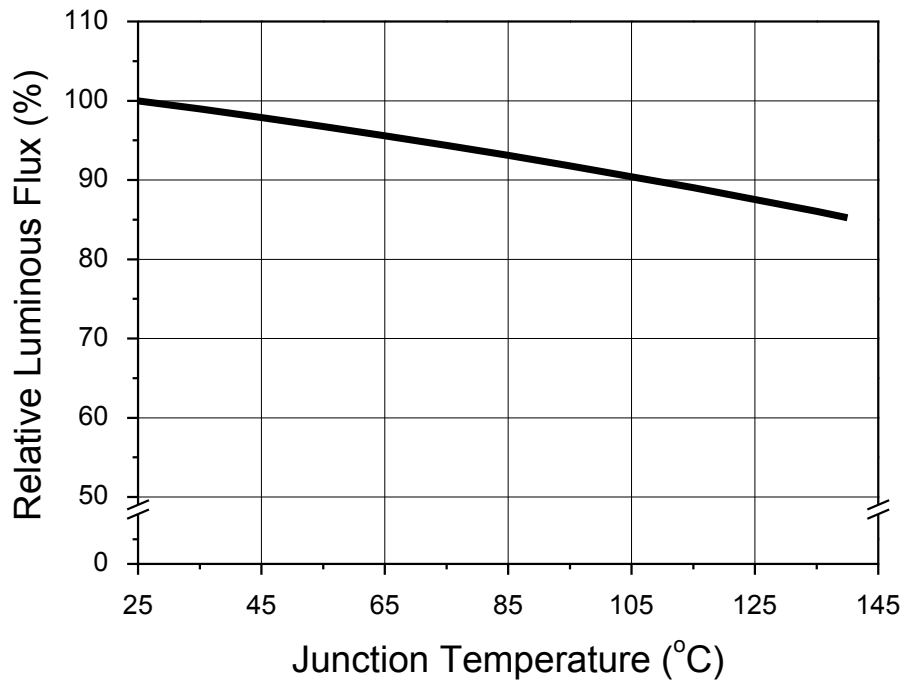
Fig 6. Junction Temperature vs. Relative Luminous Flux, I_F=0.9A
