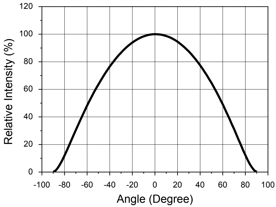
Fig 3. Radiant Pattern
